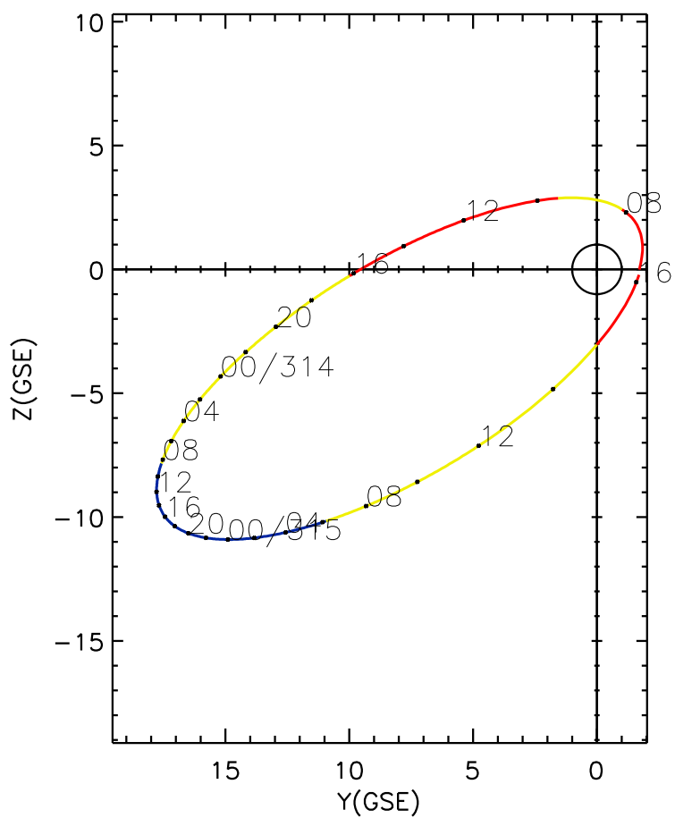
CLUSTER 2 orbit 2008 313 (11/08) 07:01 UT to 2008 315 (11/10) 16:06 UT
