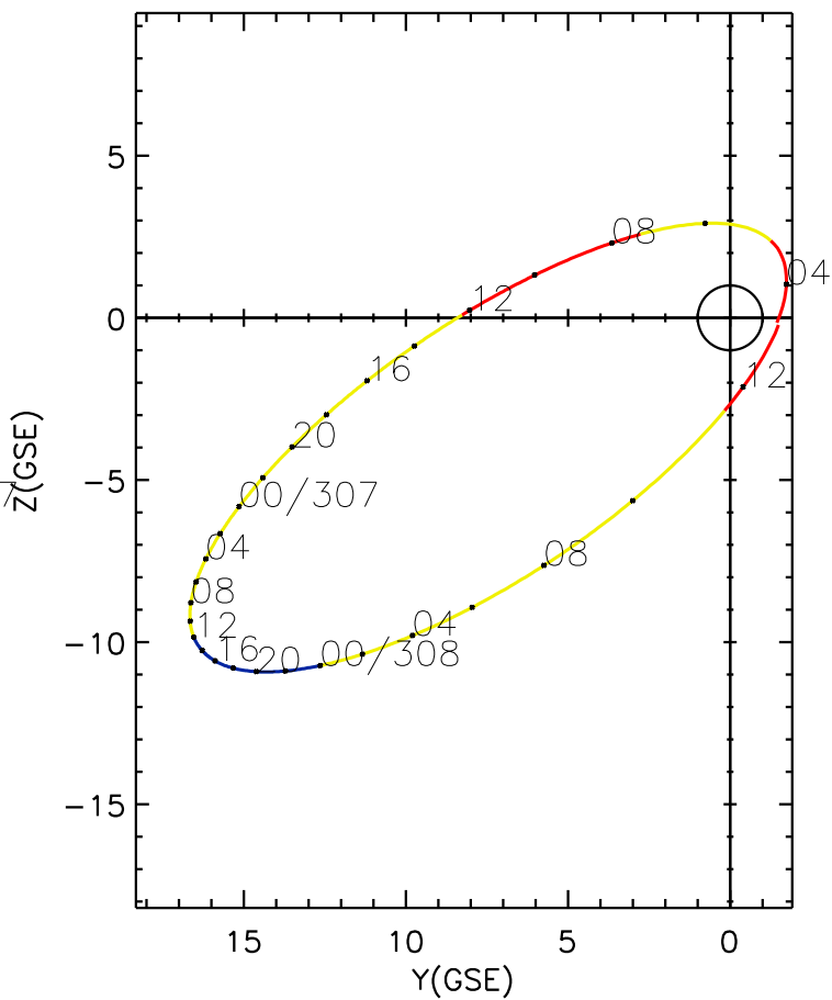
CLUSTER 2 orbit 2008 306 (11/01) 03:36 UT to 2008 308 (11/03) 12:41 UT
