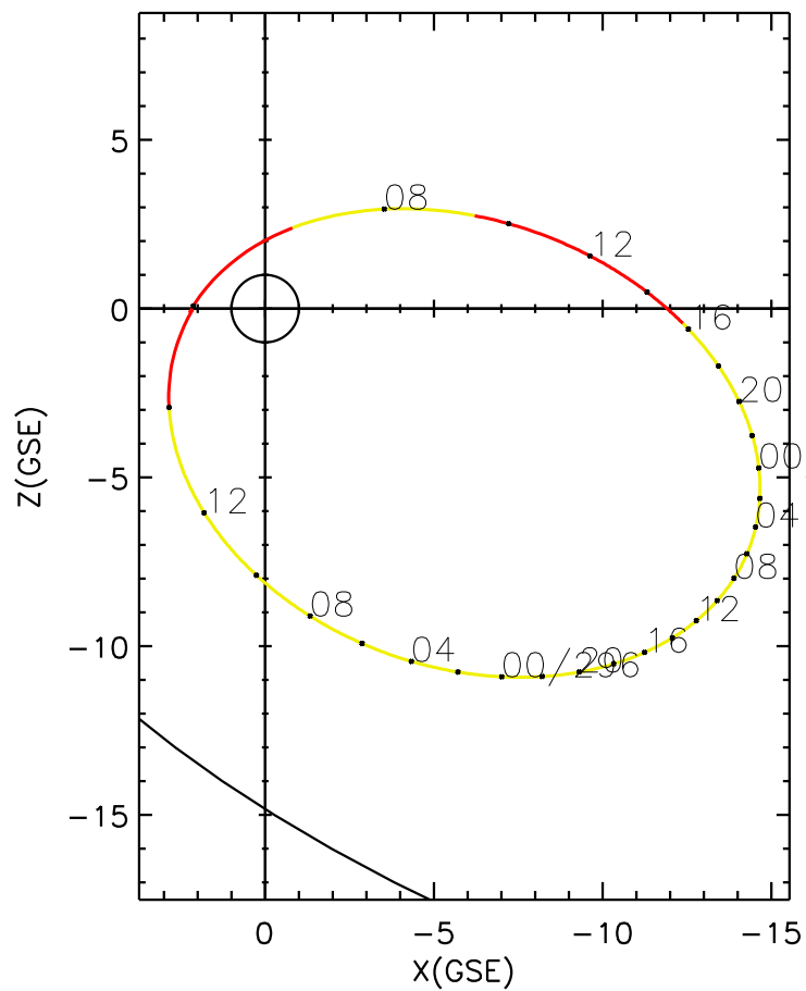
CLUSTER 2 orbit 2008 294 (10/20) 05:56 UT to 2008 296 (10/22) 15:06 UT
