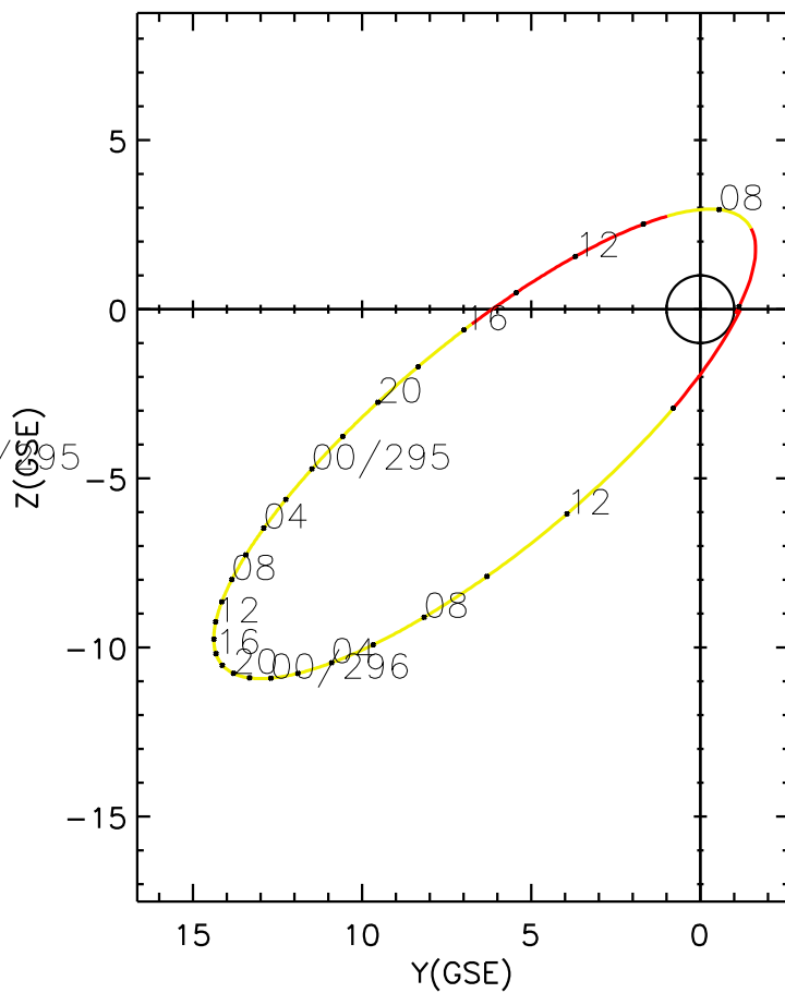
CLUSTER 2 orbit 2008 294 (10/20) 05:56 UT to 2008 296 (10/22) 15:06 UT
