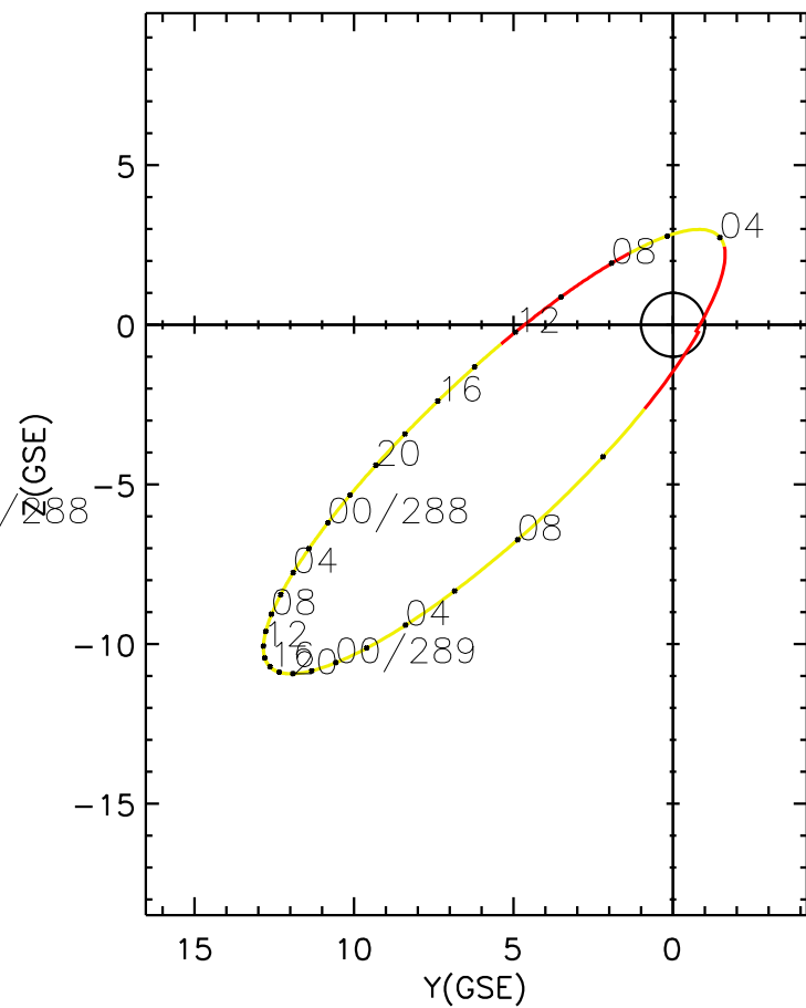
CLUSTER 2 orbit 2008 287 (10/13) 02:31 UT to 2008 289 (10/15) 11:41 UT
