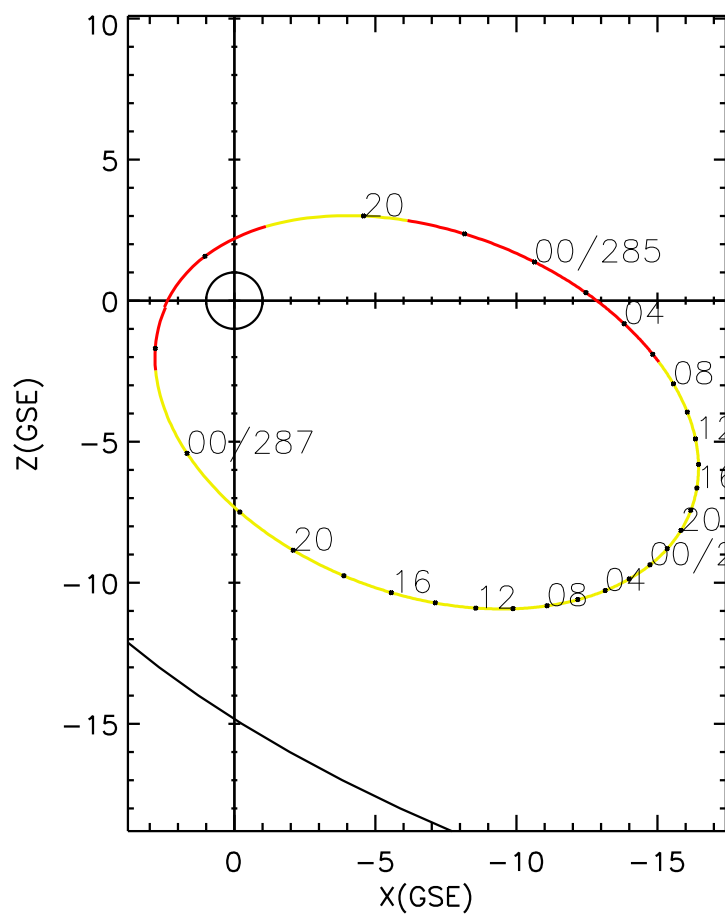
CLUSTER 2 orbit 2008 284 (10/10) 17:21 UT to 2008 287 (10/13) 02:31 UT
