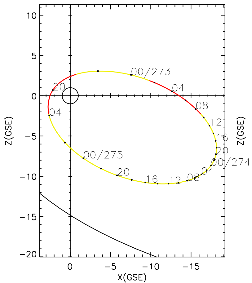
CLUSTER 2 orbit 2008 272 (09/28) 19:41 UT to 2008 275 (10/01) 04:51 UT
