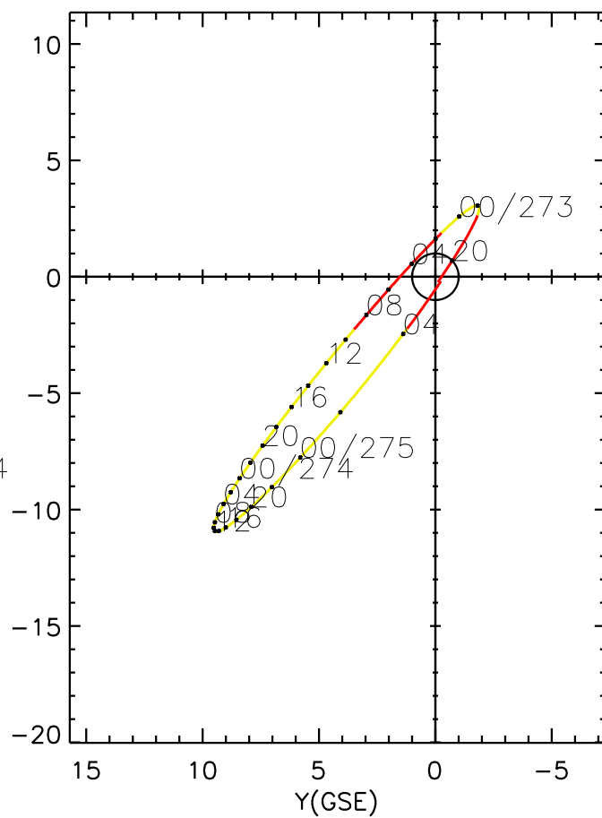
CLUSTER 2 orbit 2008 272 (09/28) 19:41 UT to 2008 275 (10/01) 04:51 UT
