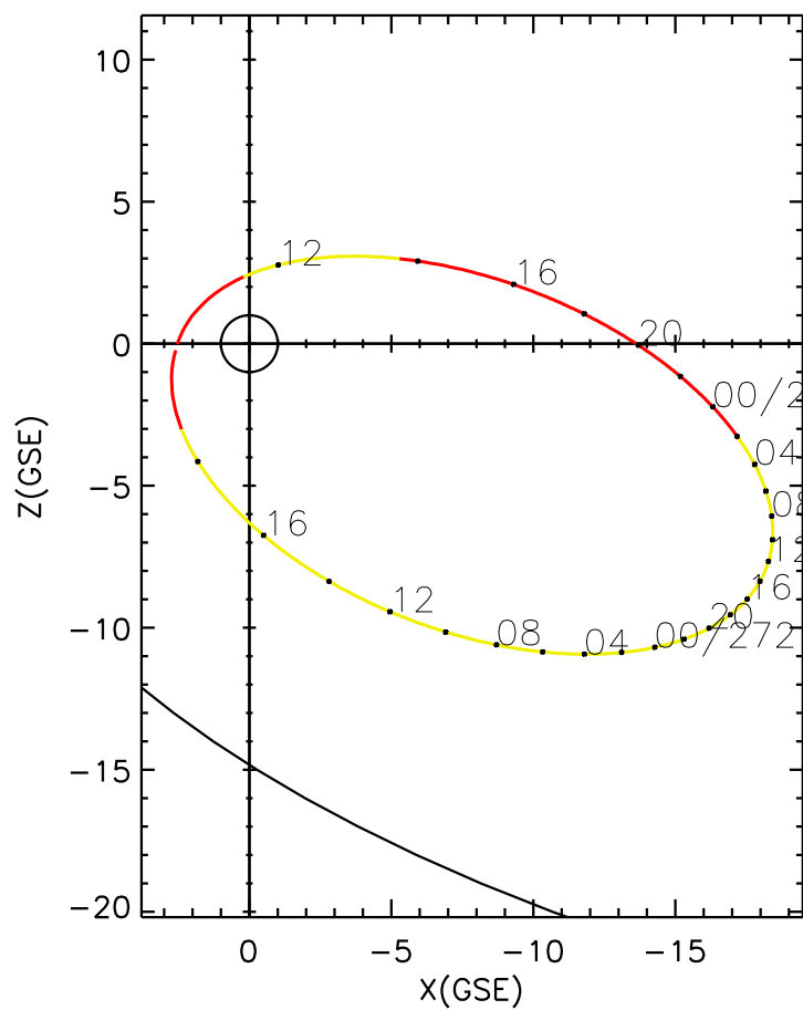
CLUSTER 2 orbit 2008 270 (09/26) 10:36 UT to 2008 272 (09/28) 19:41 UT
