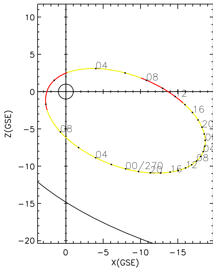
CLUSTER 2 orbit 2008 268 (09/24) 01:26 UT to 2008 270 (09/26) 10:36 UT
