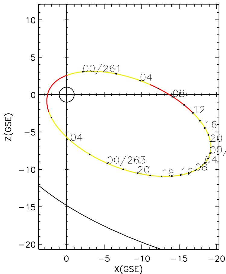
CLUSTER 2 orbit 2008 260 (09/16) 22:01 UT to 2008 263 (09/19) 07:11 UT
