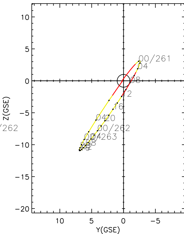
CLUSTER 2 orbit 2008 260 (09/16) 22:01 UT to 2008 263 (09/19) 07:11 UT
