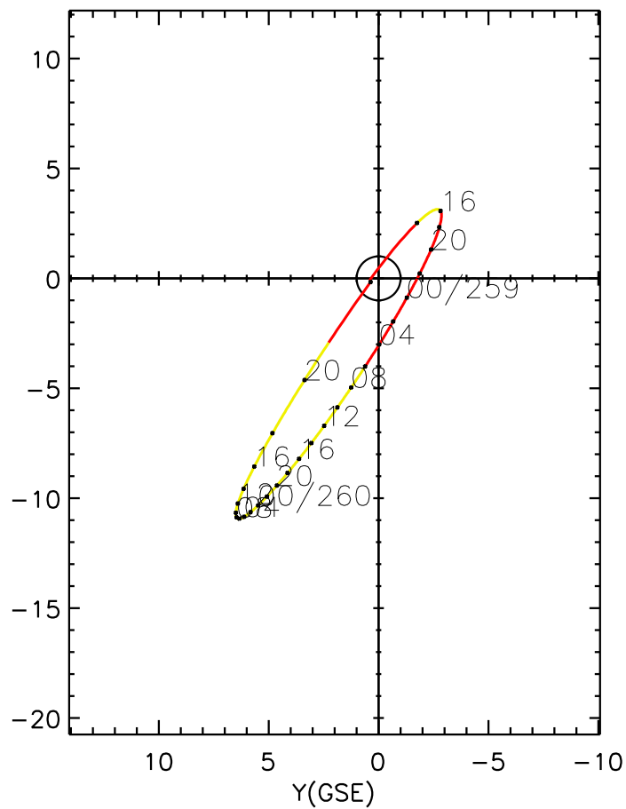
CLUSTER 2 orbit 2008 258 (09/14) 12:51 UT to 2008 260 (09/16) 22:01 UT
