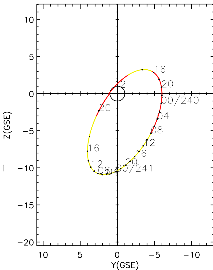
CLUSTER 2 orbit 2008 239 (08/26) 11:41 UT to 2008 241 (08/28) 20:51 UT
