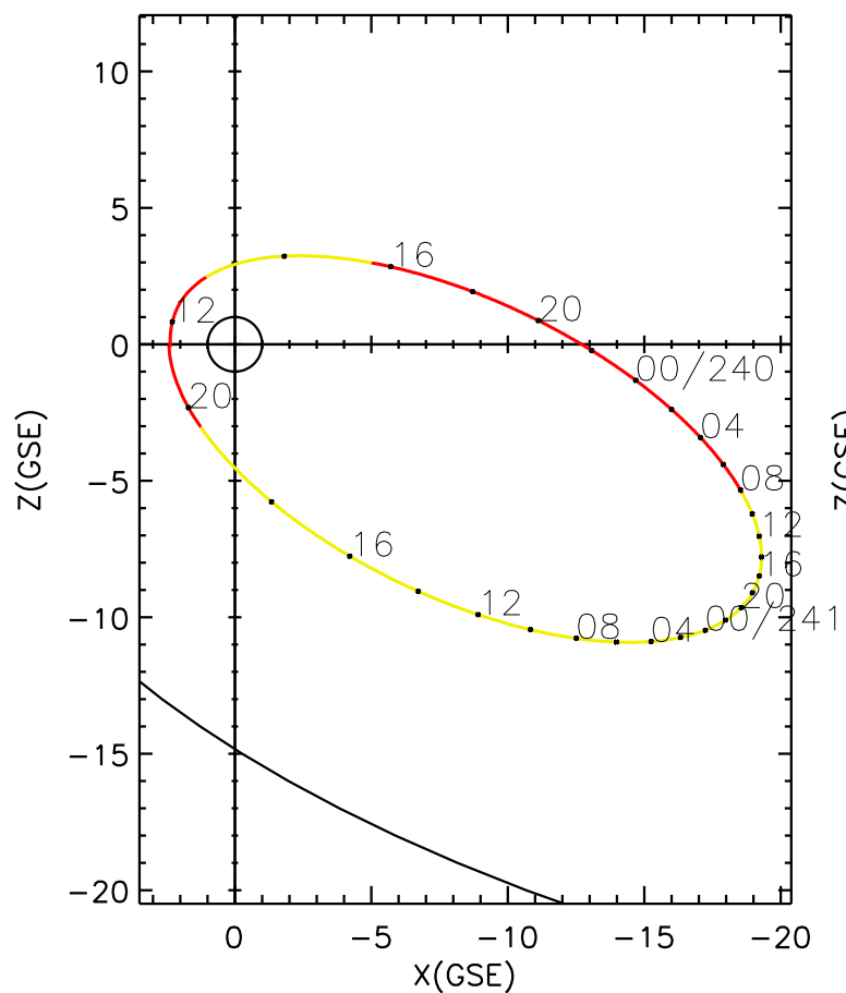
CLUSTER 2 orbit 2008 239 (08/26) 11:41 UT to 2008 241 (08/28) 20:51 UT
