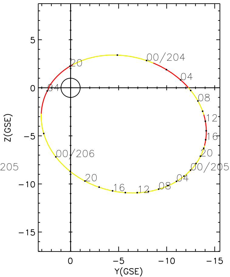
CLUSTER 2 orbit 2008 203 (07/21) 19:06 UT to 2008 206 (07/24) 04:06 UT
