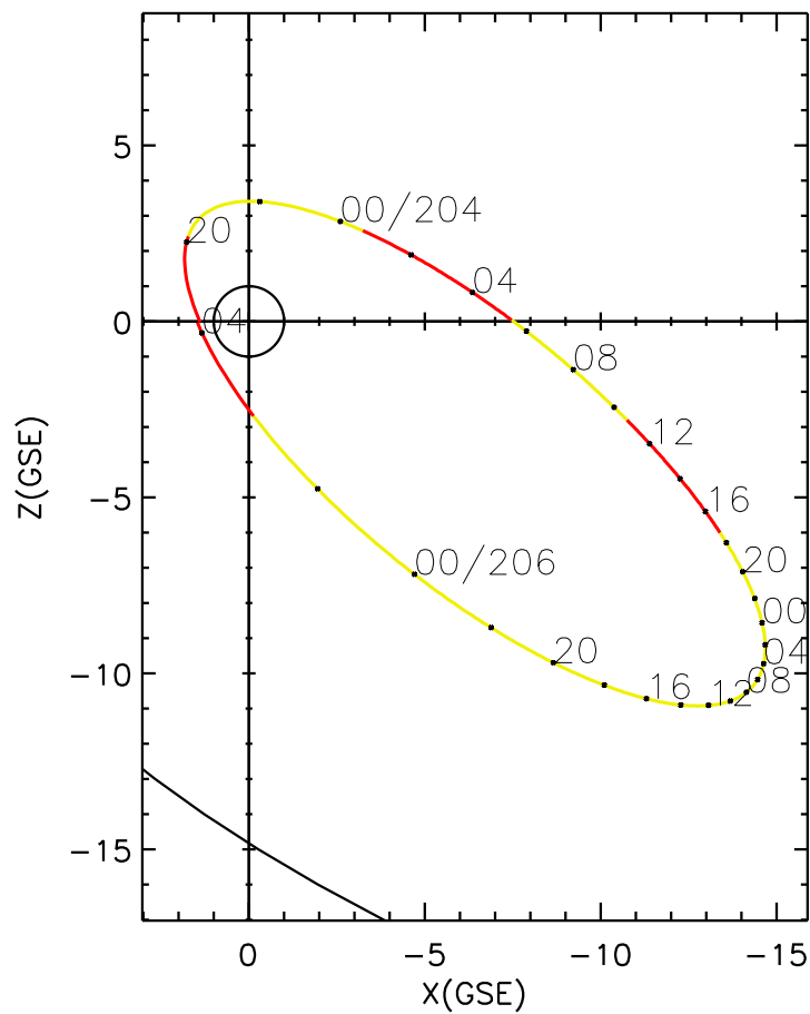
CLUSTER 2 orbit 2008 203 (07/21) 19:06 UT to 2008 206 (07/24) 04:06 UT
