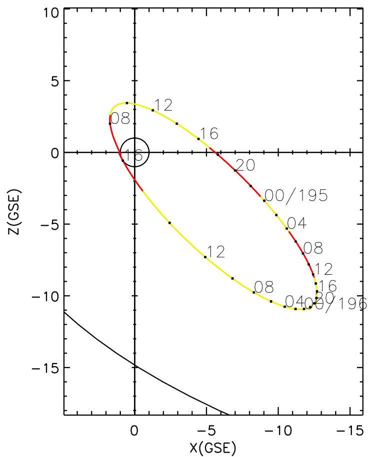
CLUSTER 2 orbit 2008 194 (07/12) 07:11 UT to 2008 196 (07/14) 16:11 UT
