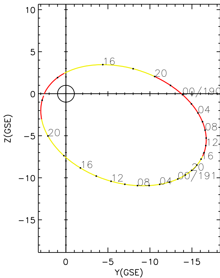
CLUSTER 2 orbit 2008 189 (07/07) 13:16 UT to 2008 191 (07/09) 22:11 UT
