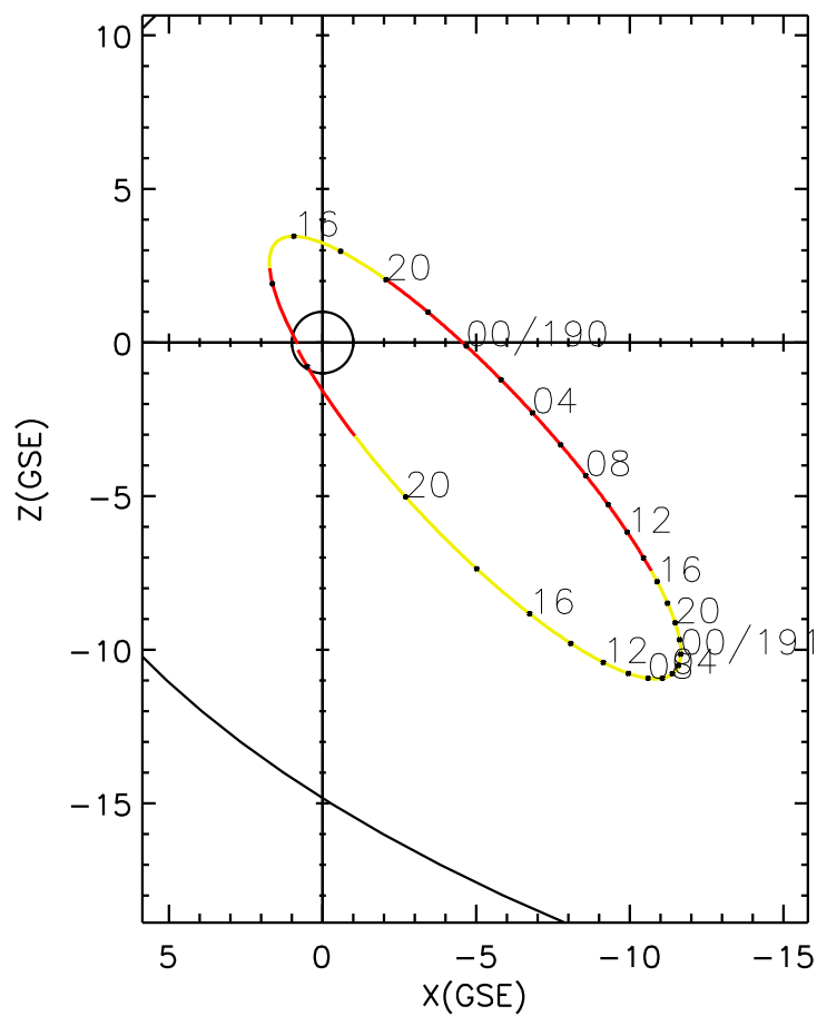
CLUSTER 2 orbit 2008 189 (07/07) 13:16 UT to 2008 191 (07/09) 22:11 UT
