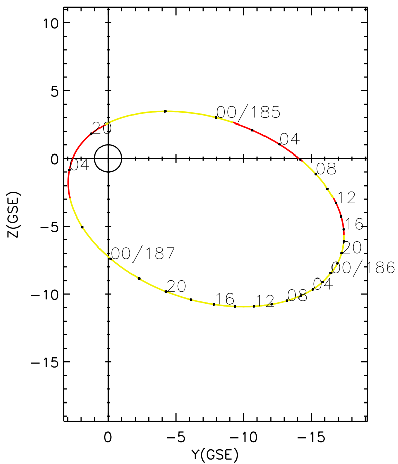
CLUSTER 2 orbit 2008 184 (07/02) 19:16 UT to 2008 187 (07/05) 04:16 UT
