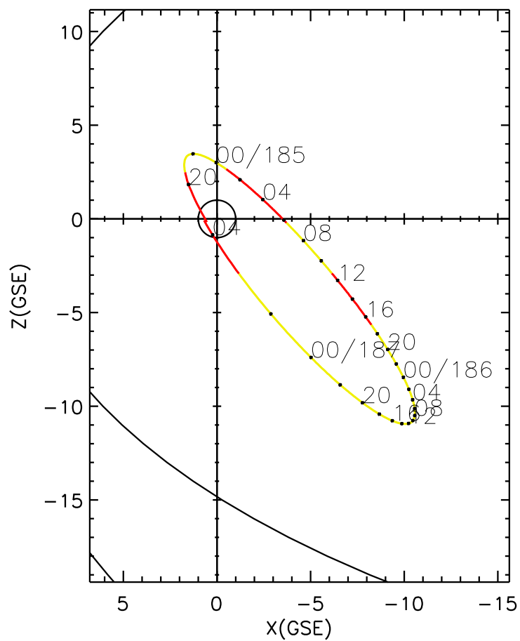
CLUSTER 2 orbit 2008 184 (07/02) 19:16 UT to 2008 187 (07/05) 04:16 UT
