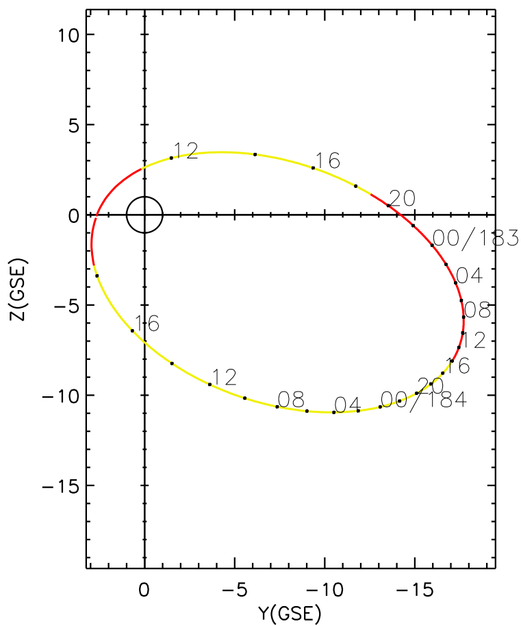
CLUSTER 2 orbit 2008 182 (06/30) 10:21 UT to 2008 184 (07/02) 19:16 UT
