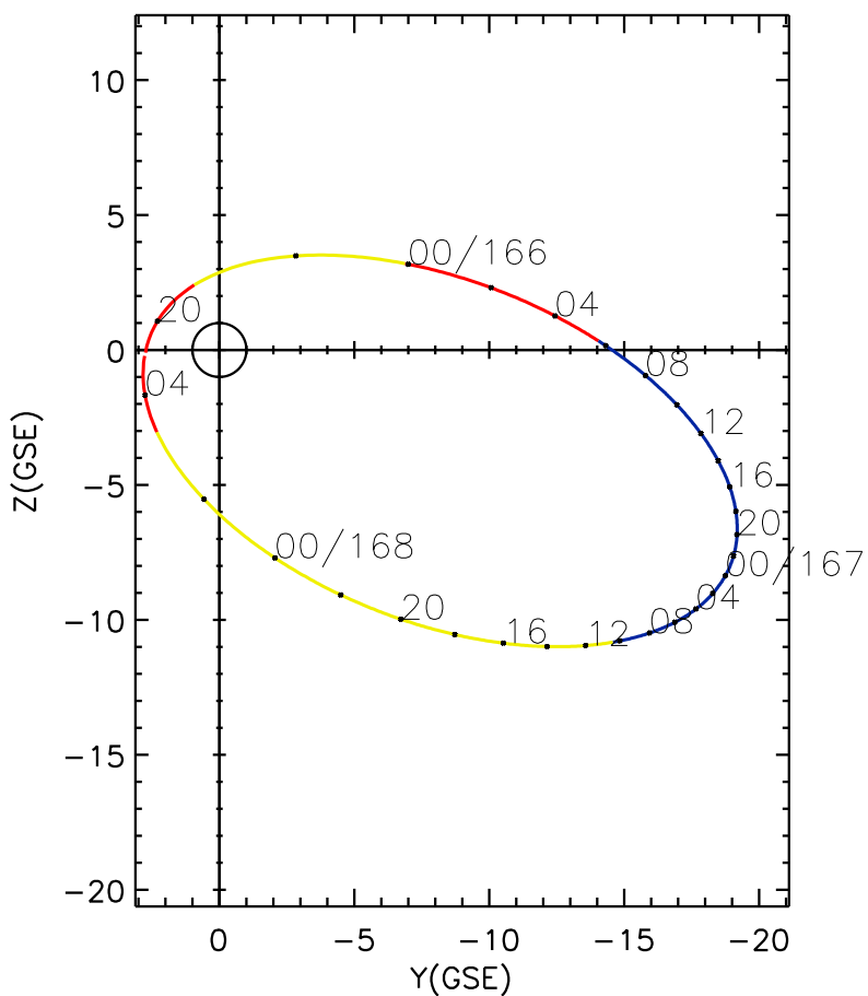
CLUSTER 2 orbit 2008 165 (06/13) 19:36 UT to 2008 168 (06/16) 04:31 UT
