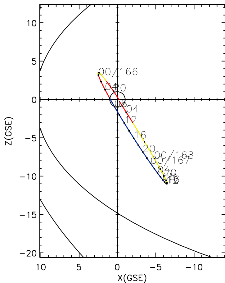
CLUSTER 2 orbit 2008 165 (06/13) 19:36 UT to 2008 168 (06/16) 04:31 UT
