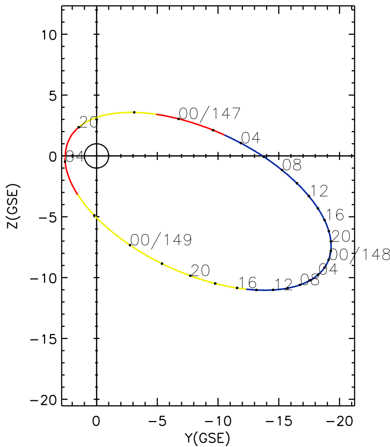
CLUSTER 2 orbit 2008 146 (05/25) 19:01 UT to 2008 149 (05/28) 04:06 UT
