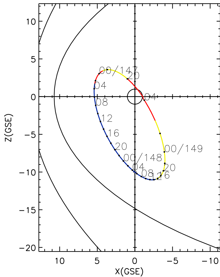
CLUSTER 2 orbit 2008 146 (05/25) 19:01 UT to 2008 149 (05/28) 04:06 UT
