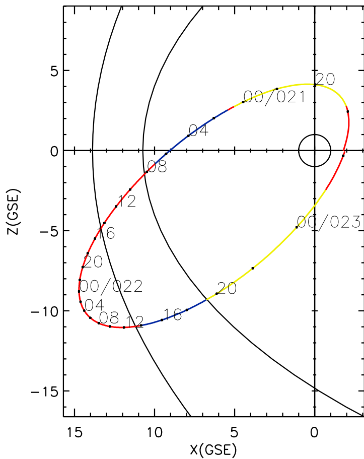
CLUSTER 2 orbit 2008 020 (01/20) 17:01 UT to 2008 023 (01/23) 02:06 UT
