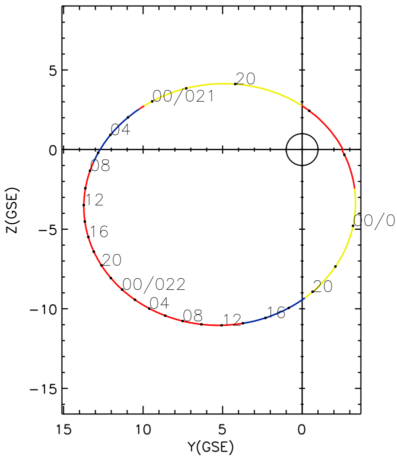
CLUSTER 2 orbit 2008 020 (01/20) 17:01 UT to 2008 023 (01/23) 02:06 UT
