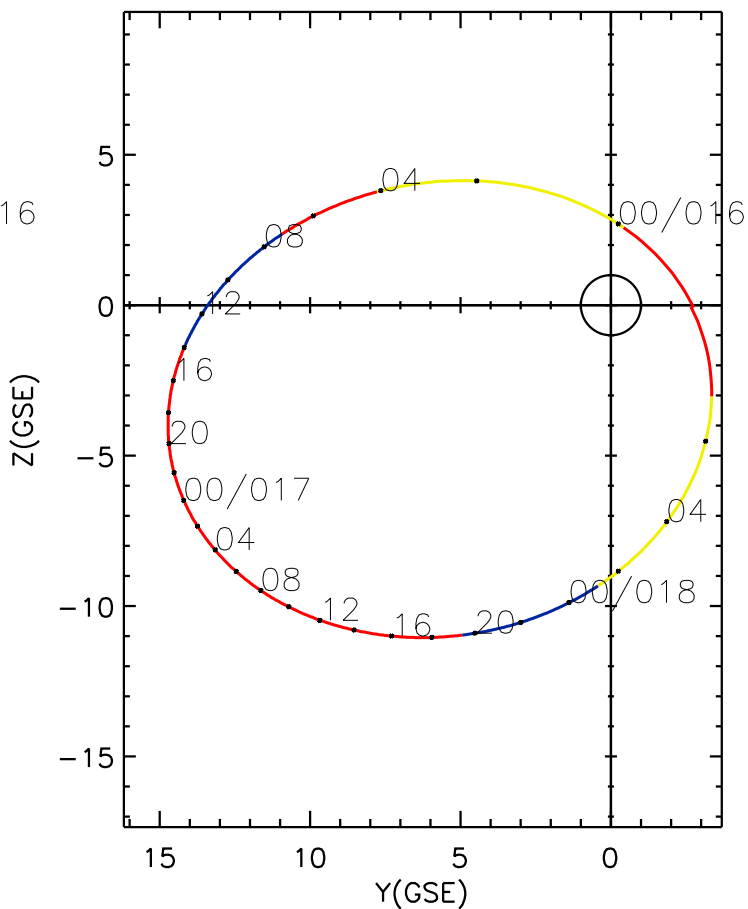
CLUSTER 2 orbit 2008 015 (01/15) 22:51 UT to 2008 018 (01/18) 07:56 UT
