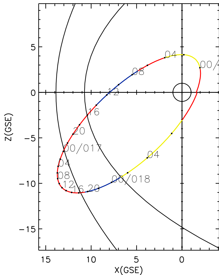
CLUSTER 2 orbit 2008 015 (01/15) 22:51 UT to 2008 018 (01/18) 07:56 UT
