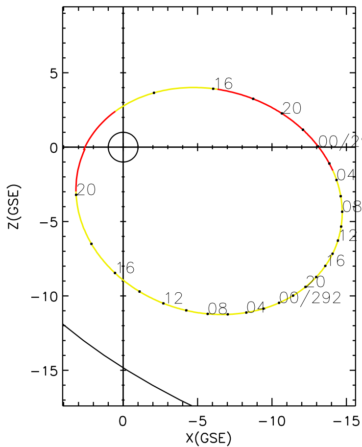
CLUSTER 2 orbit 2007 290 (10/17) 12:01 UT to 2007 292 (10/19) 21:11 UT
