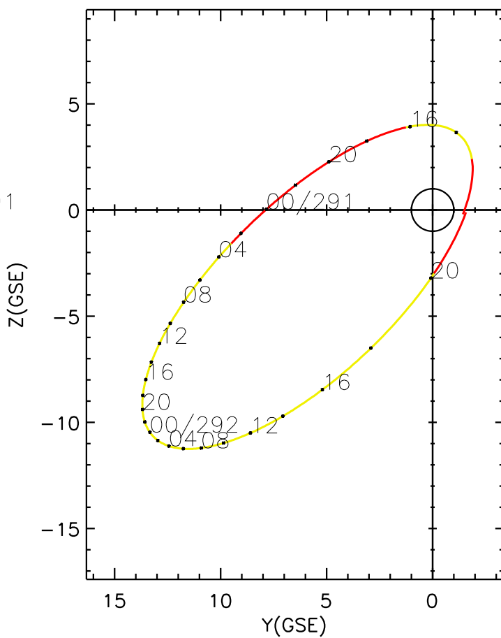
CLUSTER 2 orbit 2007 290 (10/17) 12:01 UT to 2007 292 (10/19) 21:11 UT
