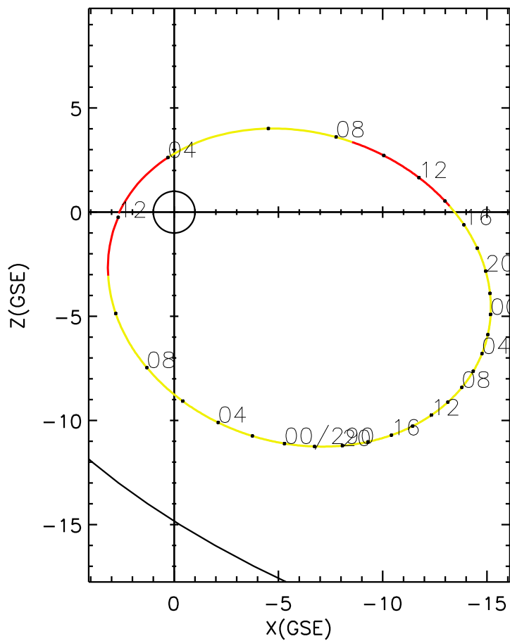
CLUSTER 2 orbit 2007 288 (10/15) 02:56 UT to 2007 290 (10/17) 12:01 UT
