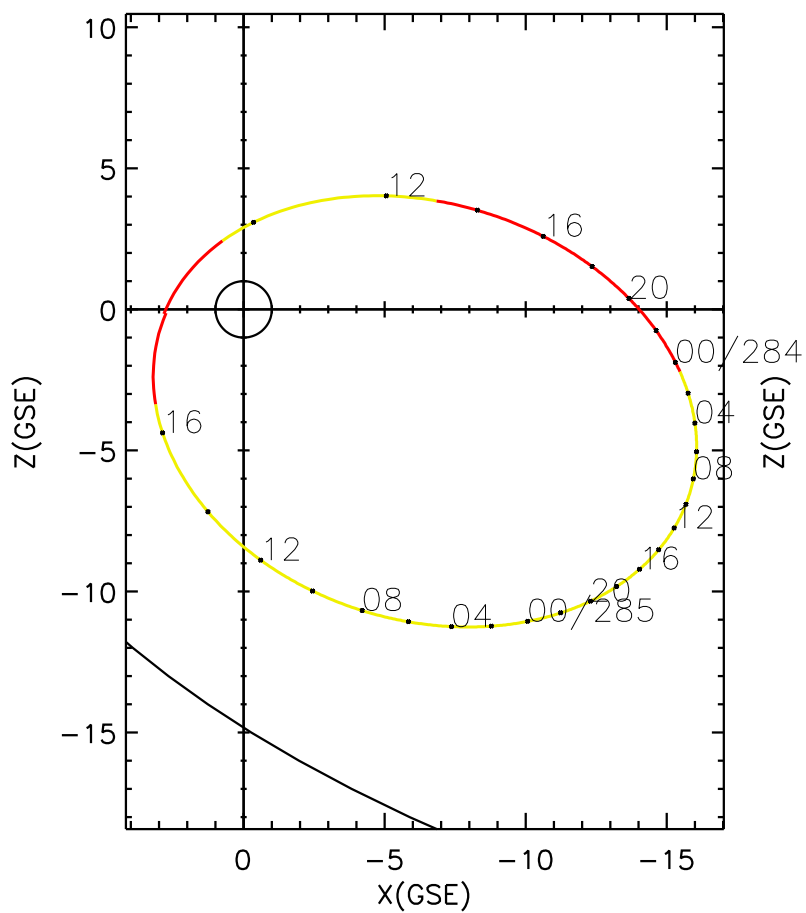
CLUSTER 2 orbit 2007 283 (10/10) 08:36 UT to 2007 285 (10/12) 17:46 UT
