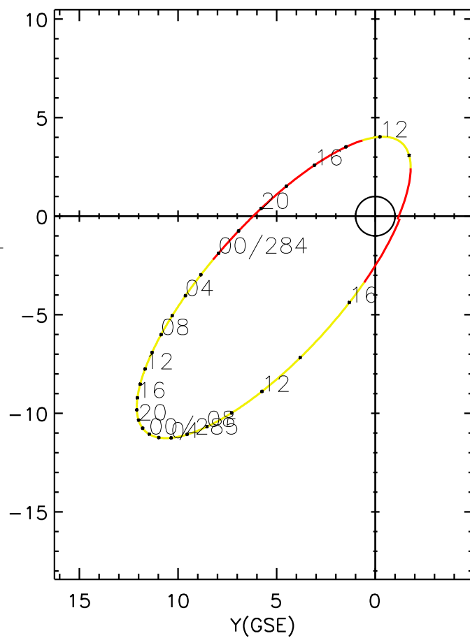
CLUSTER 2 orbit 2007 283 (10/10) 08:36 UT to 2007 285 (10/12) 17:46 UT
