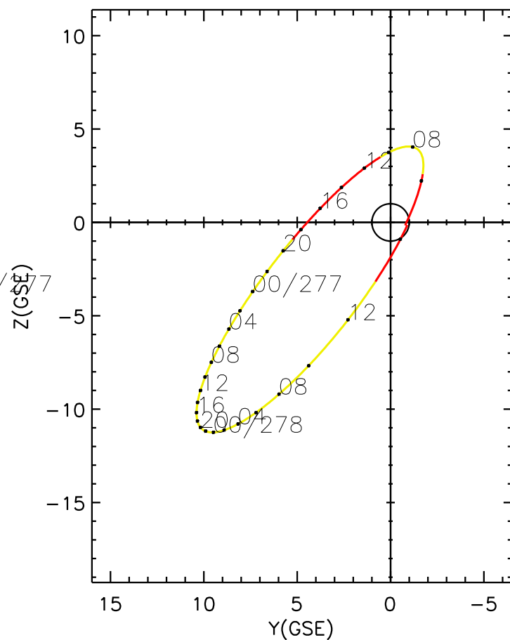
CLUSTER 2 orbit 2007 276 (10/03) 05:06 UT to 2007 278 (10/05) 14:16 UT
