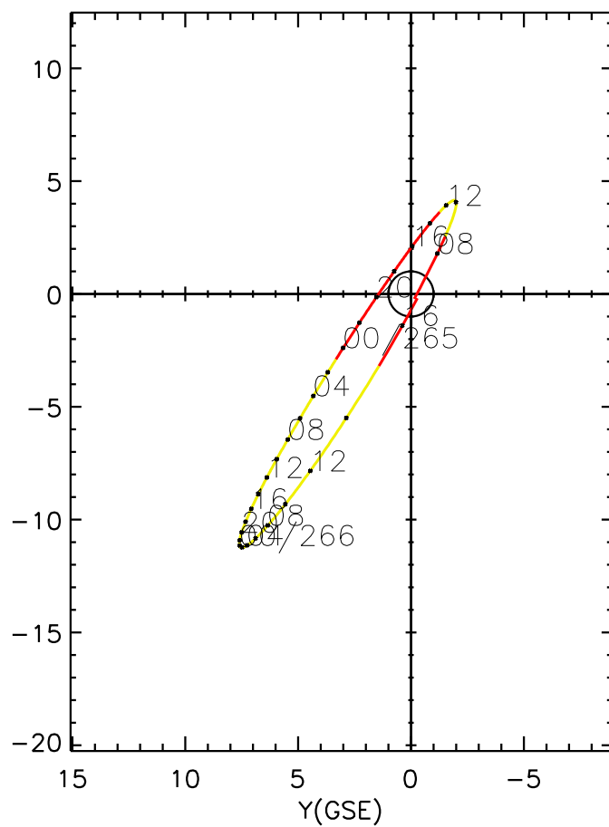
CLUSTER 2 orbit 2007 264 (09/21) 07:16 UT to 2007 266 (09/23) 16:26 UT
