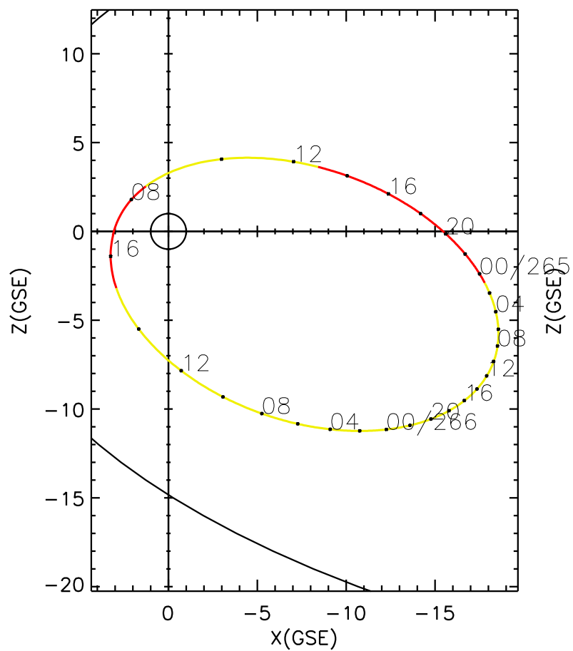
CLUSTER 2 orbit 2007 264 (09/21) 07:16 UT to 2007 266 (09/23) 16:26 UT
