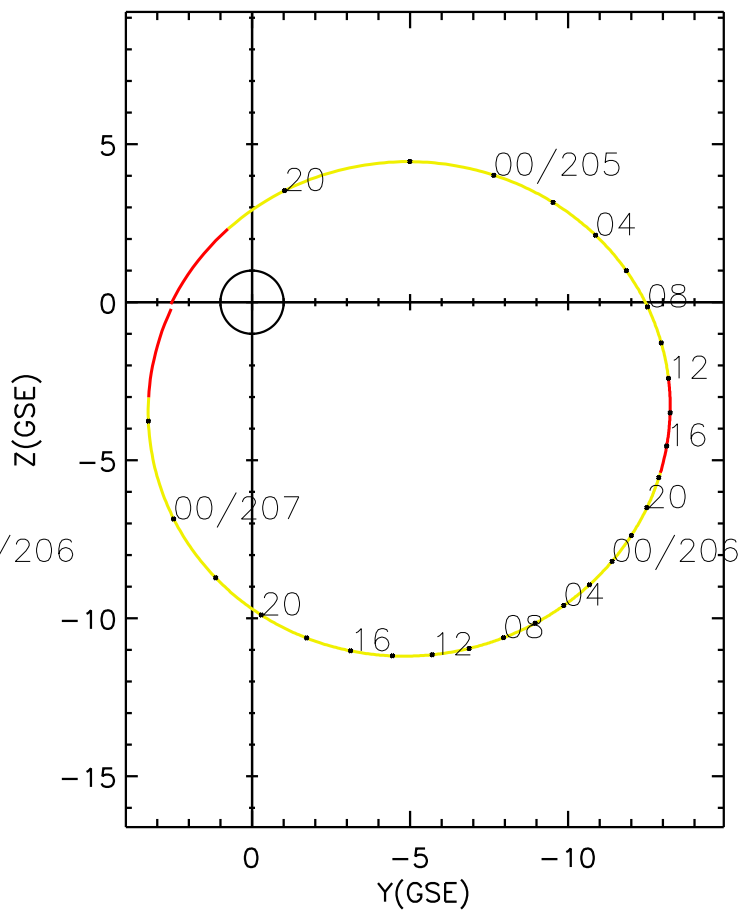
CLUSTER 2 orbit 2007 204 (07/23) 18:21 UT to 2007 207 (07/26) 03:26 UT
