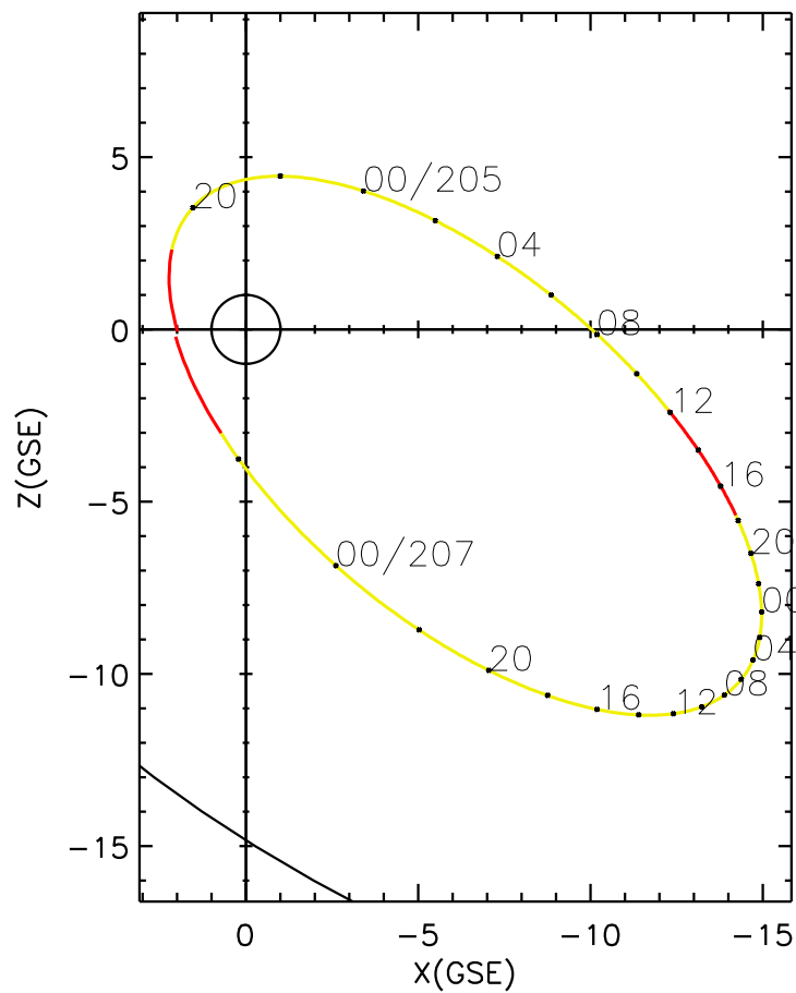
CLUSTER 2 orbit 2007 204 (07/23) 18:21 UT to 2007 207 (07/26) 03:26 UT
