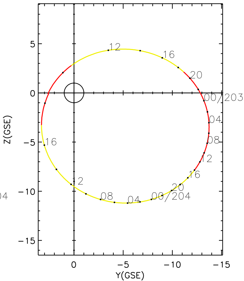
CLUSTER 2 orbit 2007 202 (07/21) 09:11 UT to 2007 204 (07/23) 18:21 UT
