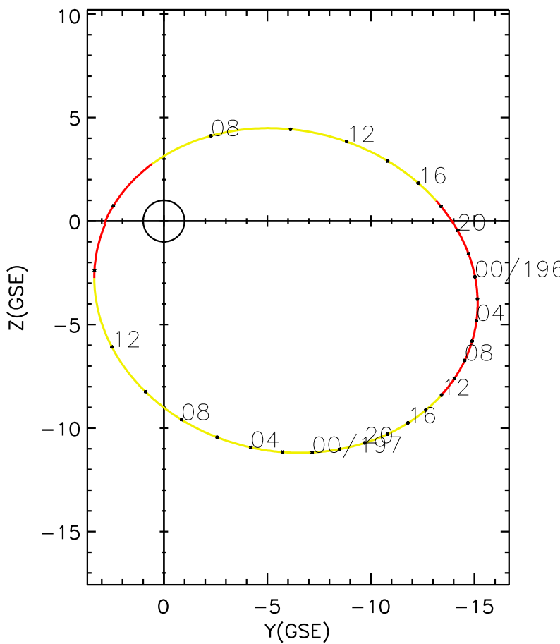
CLUSTER 2 orbit 2007 195 (07/14) 05:41 UT to 2007 197 (07/16) 14:51 UT
