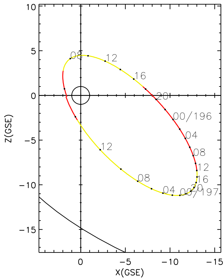
CLUSTER 2 orbit 2007 195 (07/14) 05:41 UT to 2007 197 (07/16) 14:51 UT
