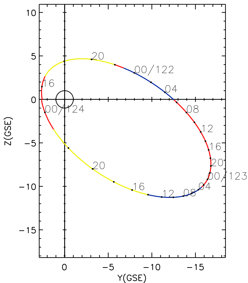
CLUSTER 2 orbit 2007 121 (05/01) 15:26 UT to 2007 124 (05/04) 00:31 UT
