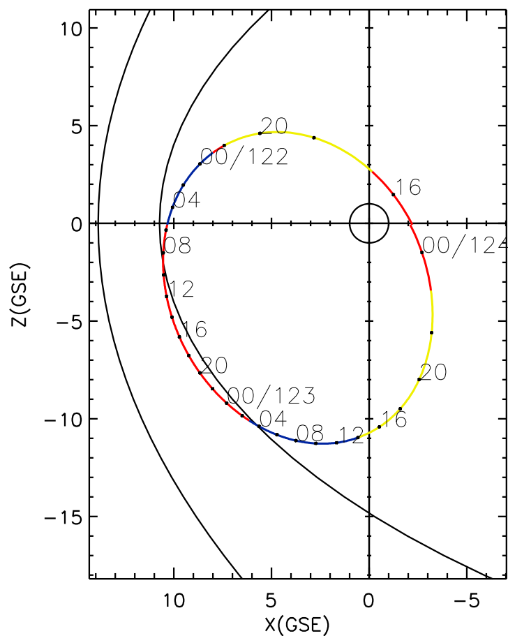
CLUSTER 2 orbit 2007 121 (05/01) 15:26 UT to 2007 124 (05/04) 00:31 UT
