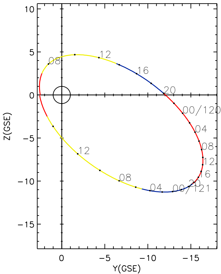
CLUSTER 2 orbit 2007 119 (04/29) 06:21 UT to 2007 121 (05/01) 15:26 UT
