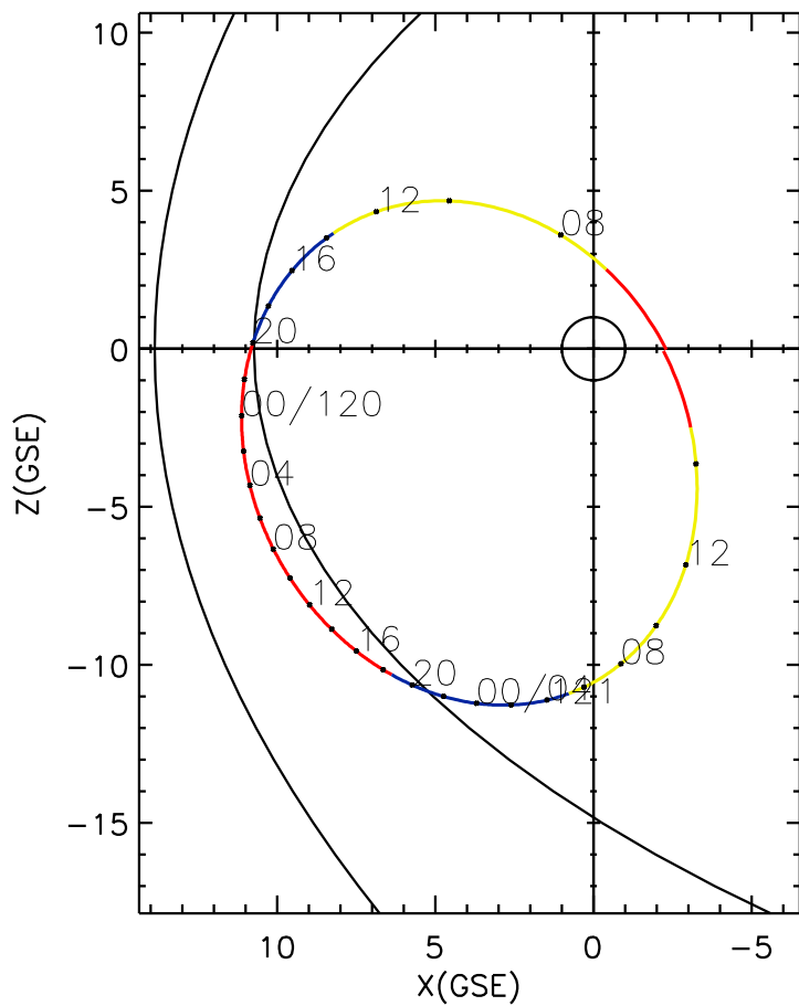
CLUSTER 2 orbit 2007 119 (04/29) 06:21 UT to 2007 121 (05/01) 15:26 UT
