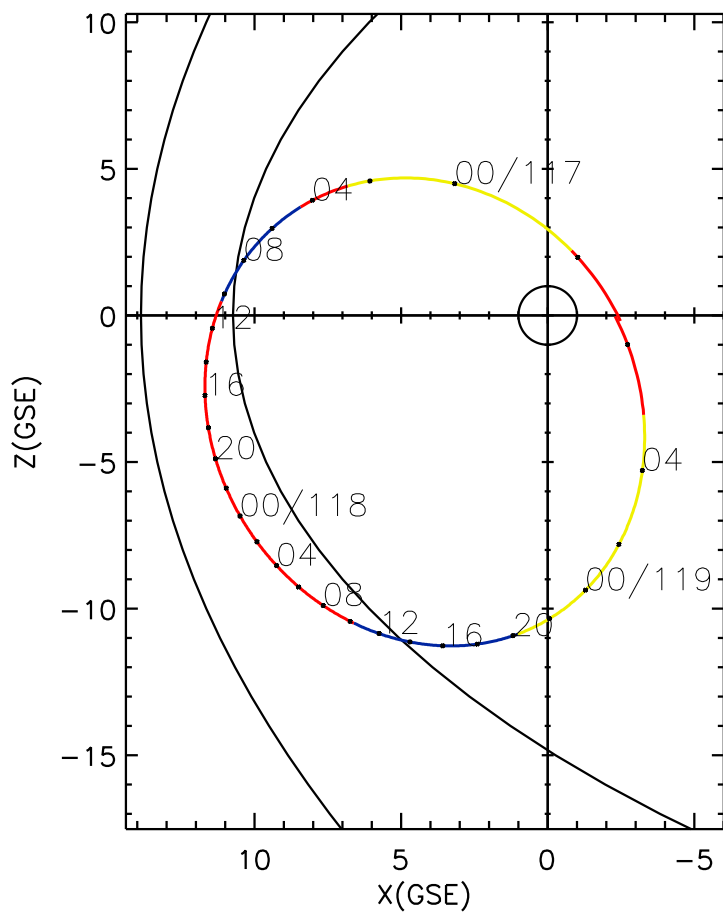
CLUSTER 2 orbit 2007 116 (04/26) 21:11 UT to 2007 119 (04/29) 06:21 UT
