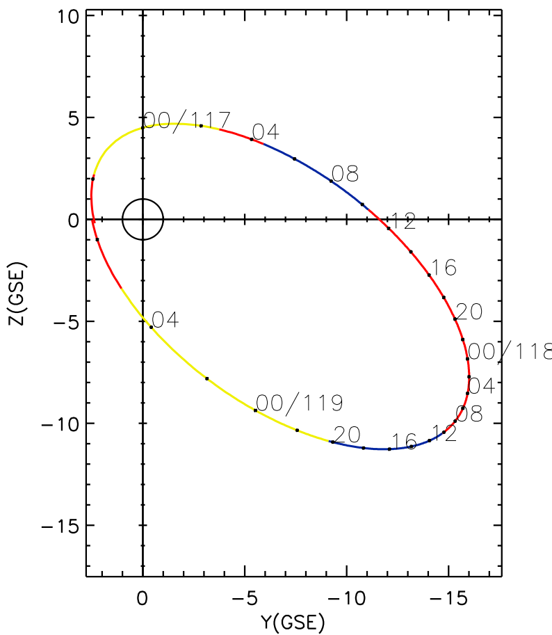
CLUSTER 2 orbit 2007 116 (04/26) 21:11 UT to 2007 119 (04/29) 06:21 UT
