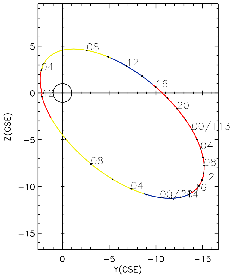
CLUSTER 2 orbit 2007 112 (04/22) 03:01 UT to 2007 114 (04/24) 12:06 UT
