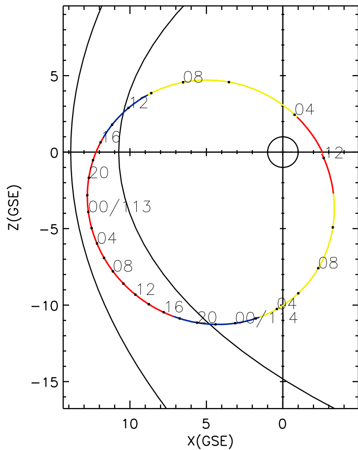
CLUSTER 2 orbit 2007 112 (04/22) 03:01 UT to 2007 114 (04/24) 12:06 UT
