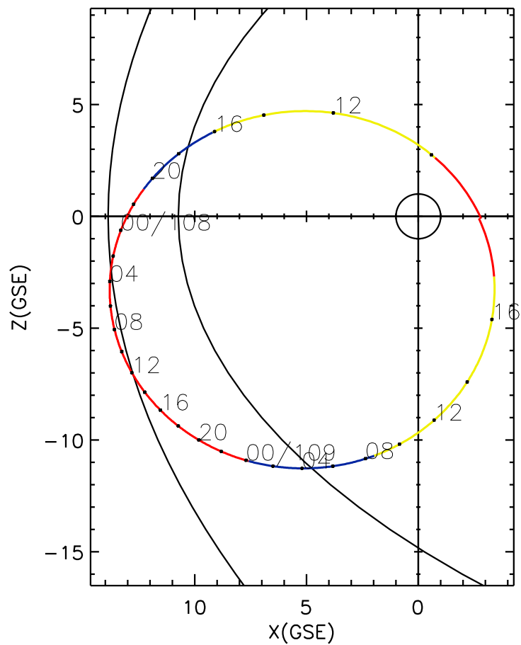
CLUSTER 2 orbit 2007 107 (04/17) 08:51 UT to 2007 109 (04/19) 17:56 UT
