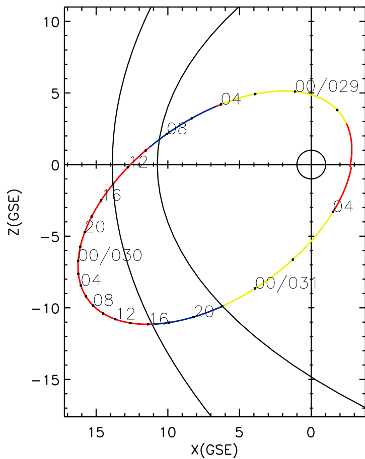
CLUSTER 2 orbit 2007 028 (01/28) 20:11 UT to 2007 031 (01/31) 05:16 UT
