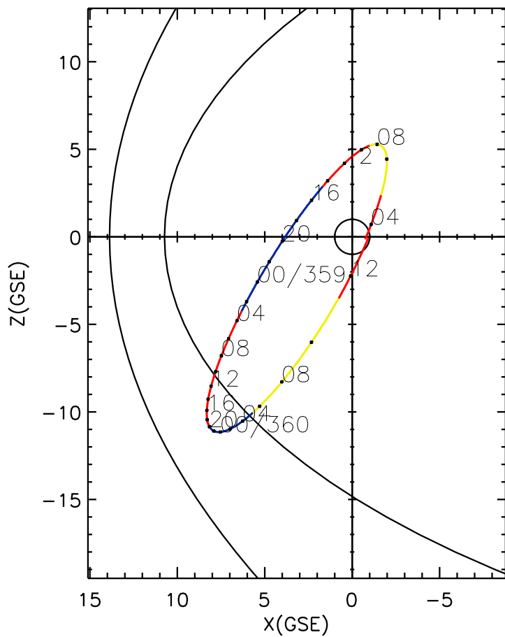
CLUSTER 2 orbit 2006 358 (12/24) 03:41 UT to 2006 360 (12/26) 12:51 UT
