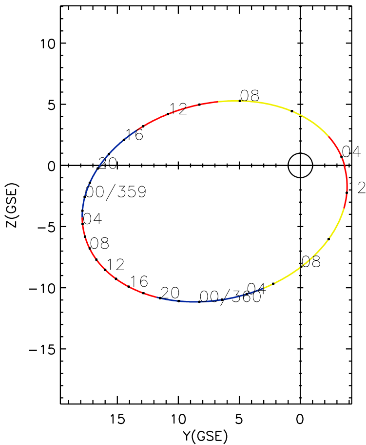
CLUSTER 2 orbit 2006 358 (12/24) 03:41 UT to 2006 360 (12/26) 12:51 UT
