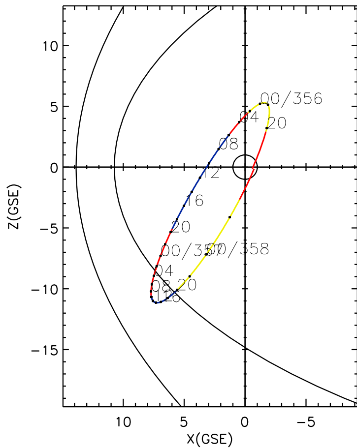
CLUSTER 2 orbit 2006 355 (12/21) 18:36 UT to 2006 358 (12/24) 03:41 UT
