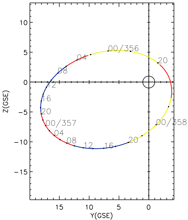
CLUSTER 2 orbit 2006 355 (12/21) 18:36 UT to 2006 358 (12/24) 03:41 UT
