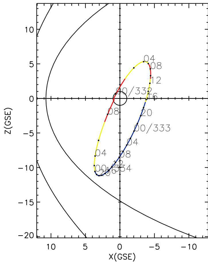
CLUSTER 2 orbit 2006 331 (11/27) 23:41 UT to 2006 334 (11/30) 08:51 UT
