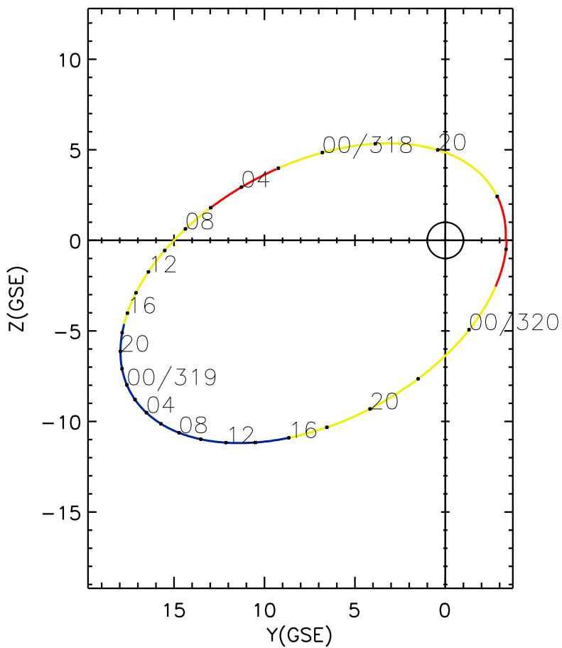
CLUSTER 2 orbit 2006 317 (11/13) 17:01 UT to 2006 320 (11/16) 02:11 UT
