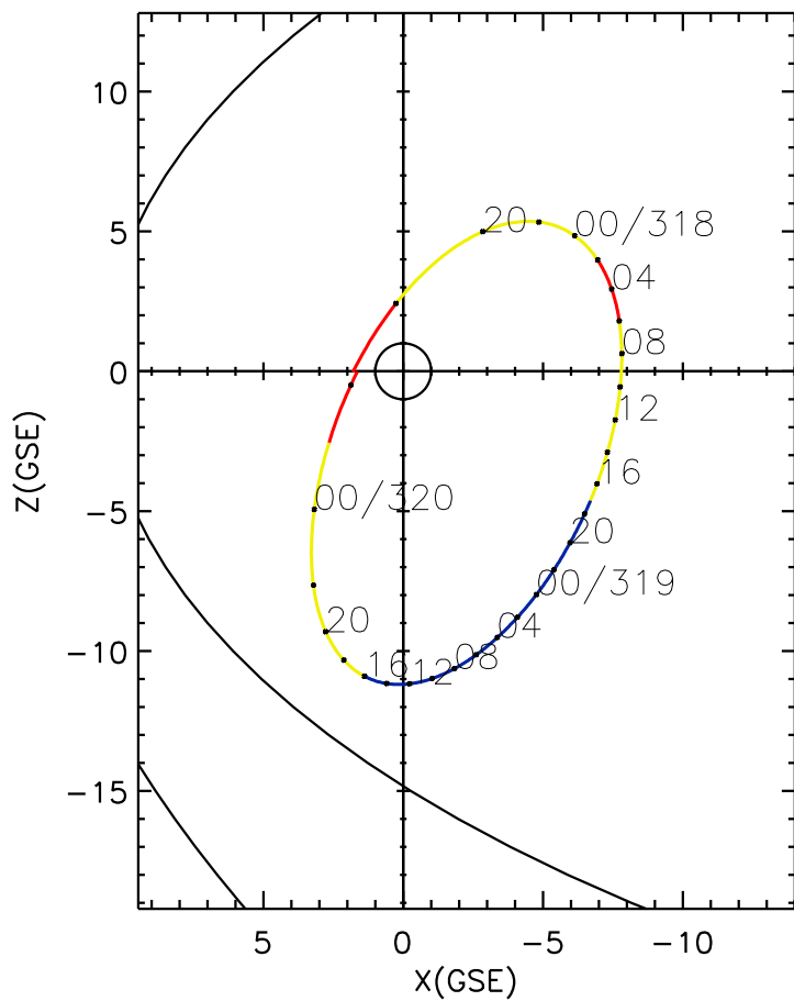
CLUSTER 2 orbit 2006 317 (11/13) 17:01 UT to 2006 320 (11/16) 02:11 UT
