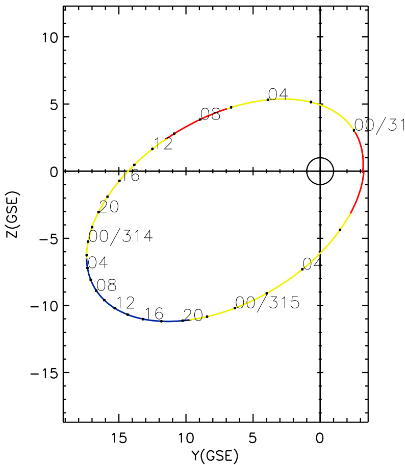
CLUSTER 2 orbit 2006 312 (11/08) 22:41 UT to 2006 315 (11/11) 07:51 UT
