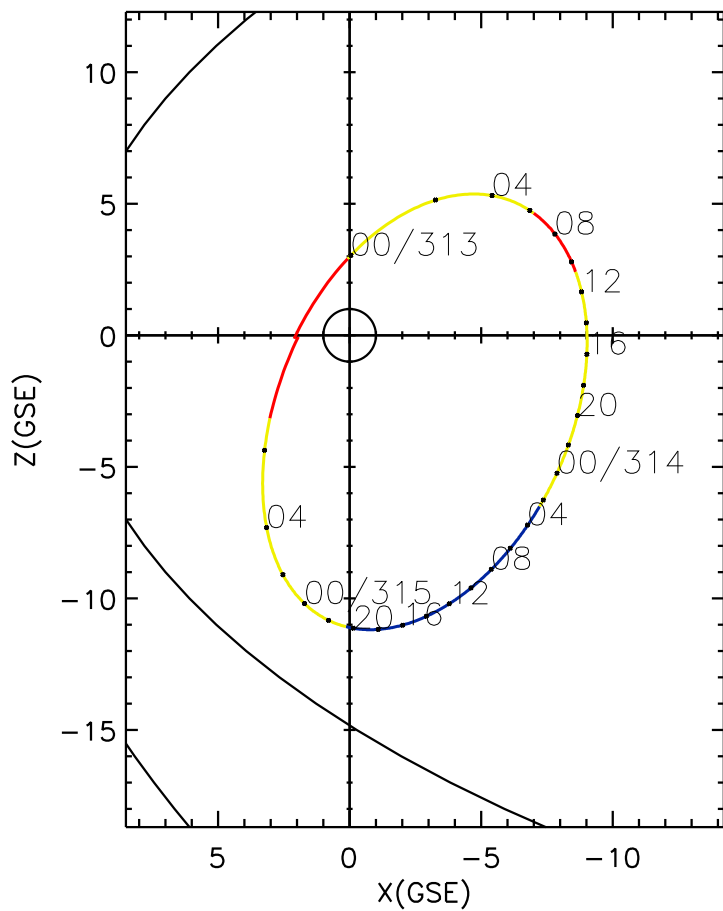
CLUSTER 2 orbit 2006 312 (11/08) 22:41 UT to 2006 315 (11/11) 07:51 UT
