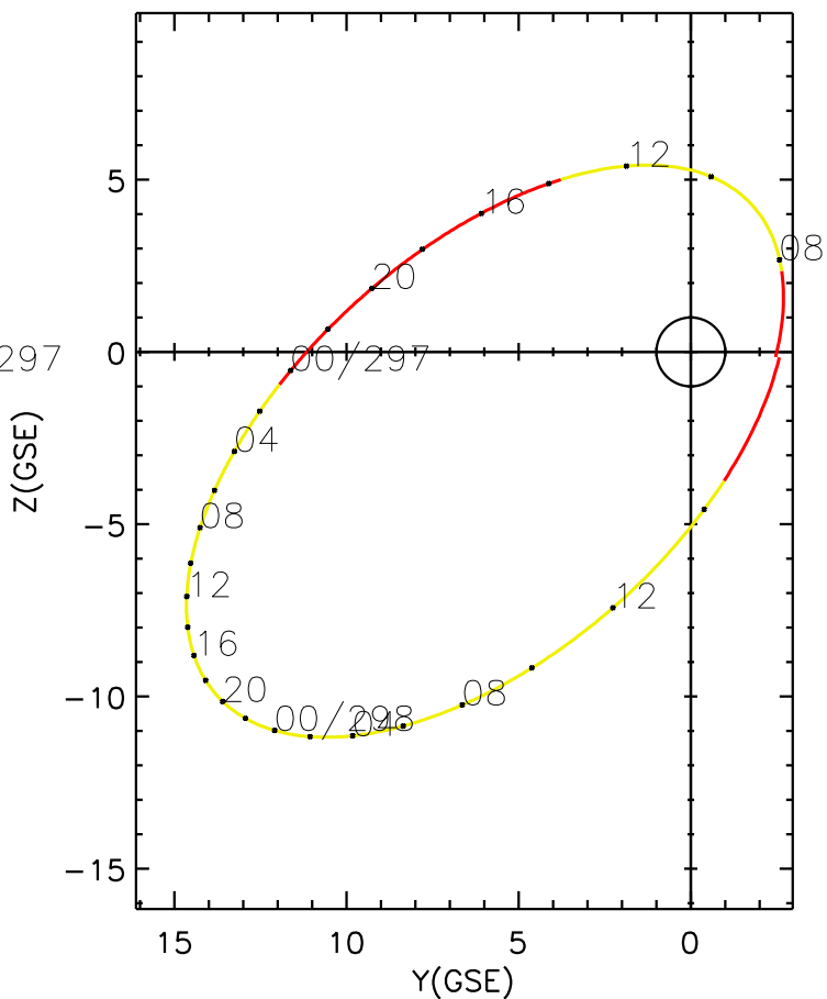
CLUSTER 2 orbit 2006 296 (10/23) 06:51 UT to 2006 298 (10/25) 15:56 UT
