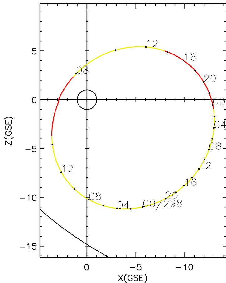
CLUSTER 2 orbit 2006 296 (10/23) 06:51 UT to 2006 298 (10/25) 15:56 UT
