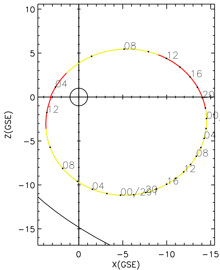
CLUSTER 2 orbit 2006 289 (10/16) 03:31 UT to 2006 291 (10/18) 12:41 UT
