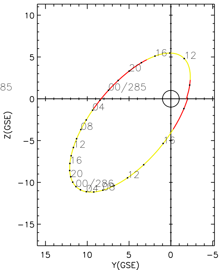
CLUSTER 2 orbit 2006 284 (10/11) 09:21 UT to 2006 286 (10/13) 18:26 UT
