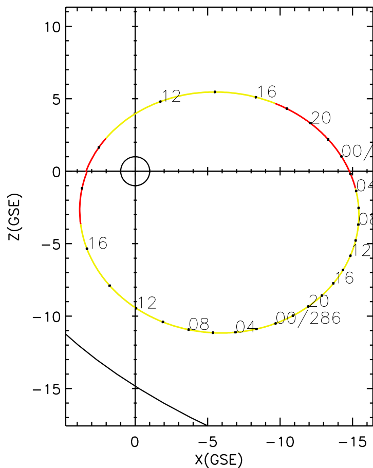
CLUSTER 2 orbit 2006 284 (10/11) 09:21 UT to 2006 286 (10/13) 18:26 UT
