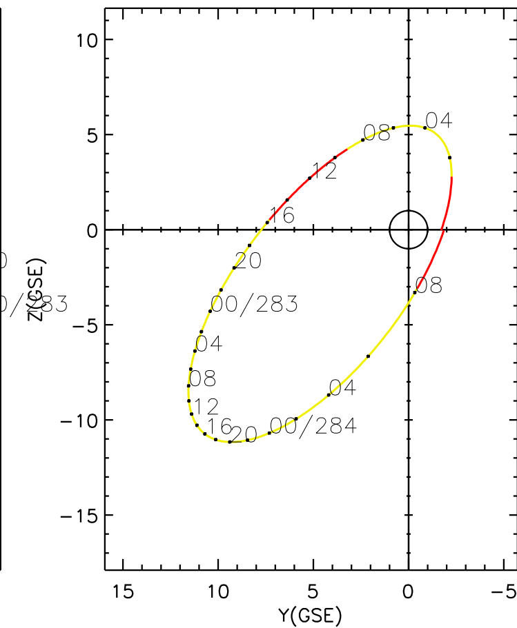
CLUSTER 2 orbit 2006 282 (10/09) 00:16 UT to 2006 284 (10/11) 09:21 UT
