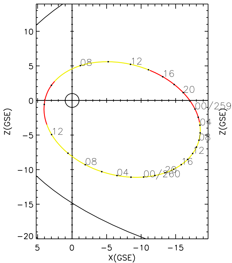
CLUSTER 2 orbit 2006 258 (09/15) 05:06 UT to 2006 260 (09/17) 14:11 UT
