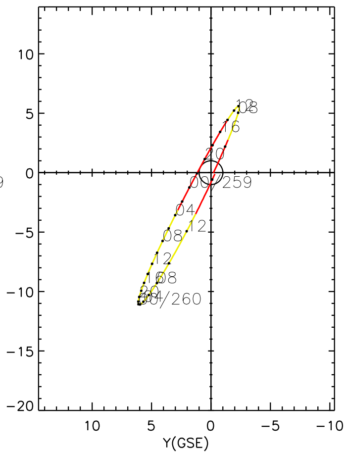
CLUSTER 2 orbit 2006 258 (09/15) 05:06 UT to 2006 260 (09/17) 14:11 UT
