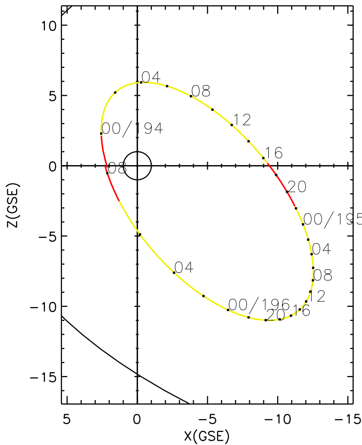
CLUSTER 2 orbit 2006 193 (07/12) 23:01 UT to 2006 196 (07/15) 08:11 UT
