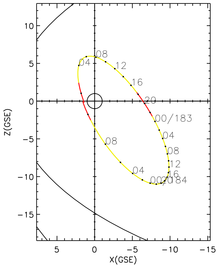
CLUSTER 2 orbit 2006 182 (07/01) 01:31 UT to 2006 184 (07/03) 10:41 UT
