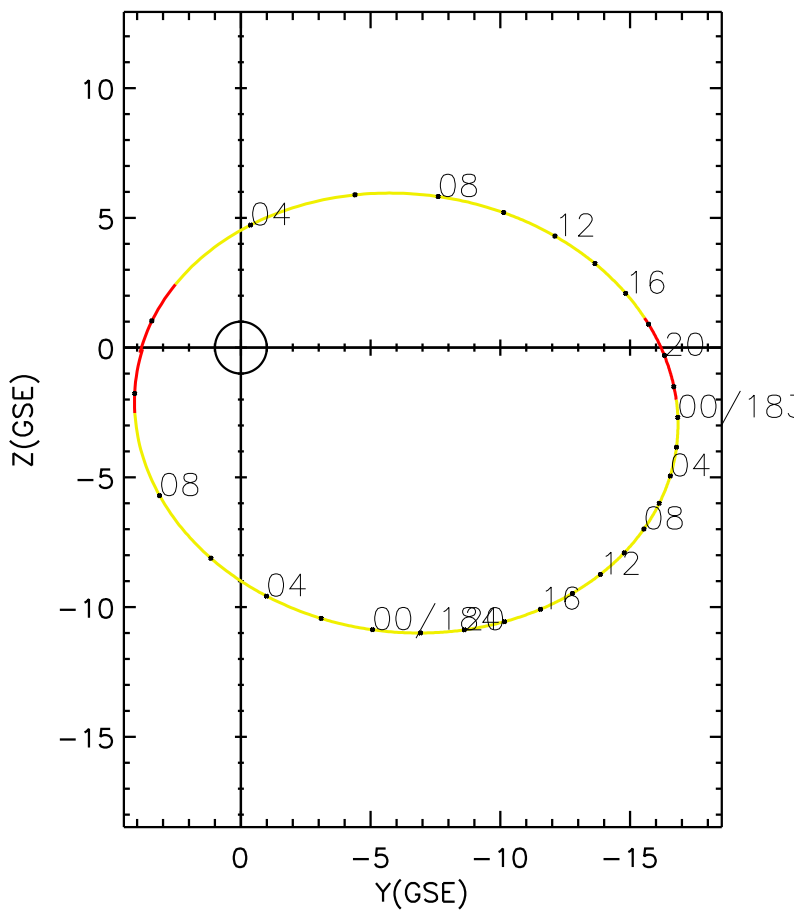
CLUSTER 2 orbit 2006 182 (07/01) 01:31 UT to 2006 184 (07/03) 10:41 UT
