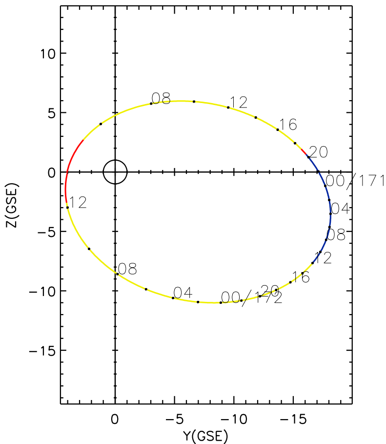
CLUSTER 2 orbit 2006 170 (06/19) 04:06 UT to 2006 172 (06/21) 13:11 UT
