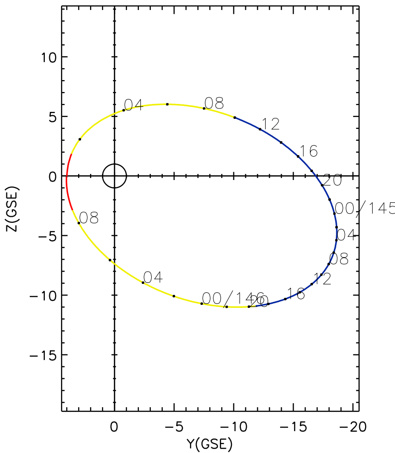
CLUSTER 2 orbit 2006 144 (05/24) 00:41 UT to 2006 146 (05/26) 09:41 UT
