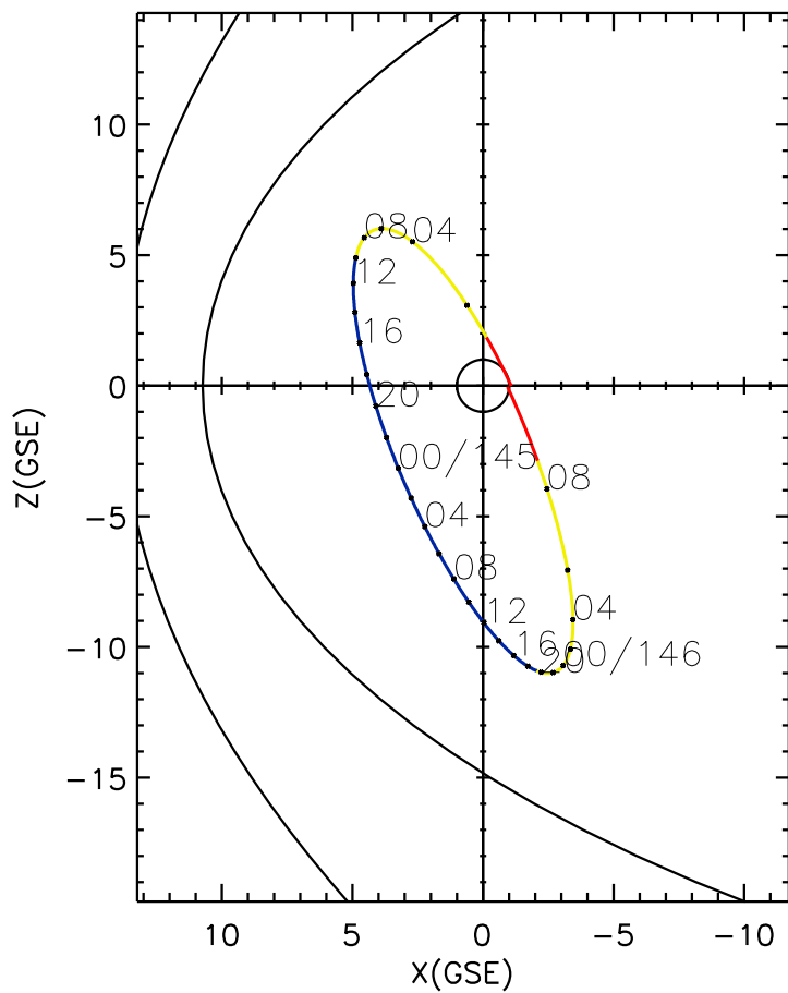
CLUSTER 2 orbit 2006 144 (05/24) 00:41 UT to 2006 146 (05/26) 09:41 UT
