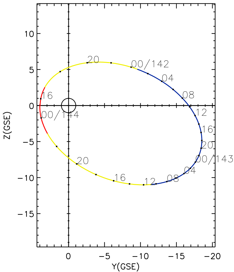
CLUSTER 2 orbit 2006 141 (05/21) 15:36 UT to 2006 144 (05/24) 00:41 UT
