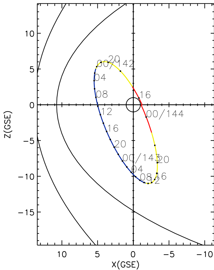
CLUSTER 2 orbit 2006 141 (05/21) 15:36 UT to 2006 144 (05/24) 00:41 UT
