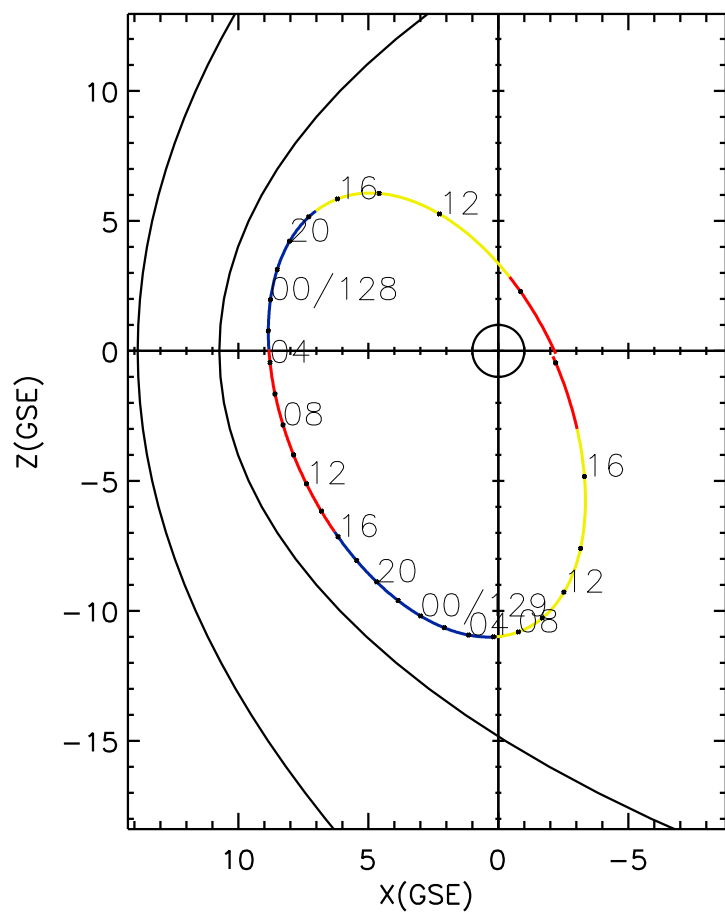
CLUSTER 2 orbit 2006 127 (05/07) 09:01 UT to 2006 129 (05/09) 18:06 UT
